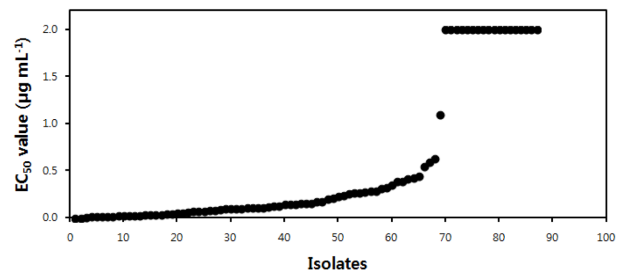
Fig. 2. Distribution of \text{EC}_{50} values of Botrytis cinerea isolates. The response of Botrytis cinerea was investigated on FGA medium amended with mepanipyrim to the each indicated concentration.
