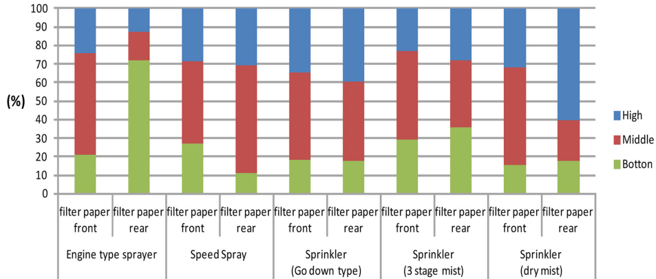
Fig. 3. Spray deposit percentile of font and rear attached filter papers by height on citrus leaves.
